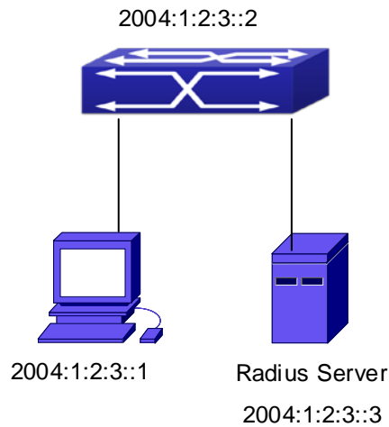
Figure 52-3-2 The Topology of IPv6 Radius configuration
