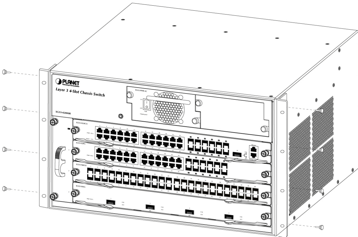
Figure 2-2-2 Attach brackets to the Chassis Switch.
