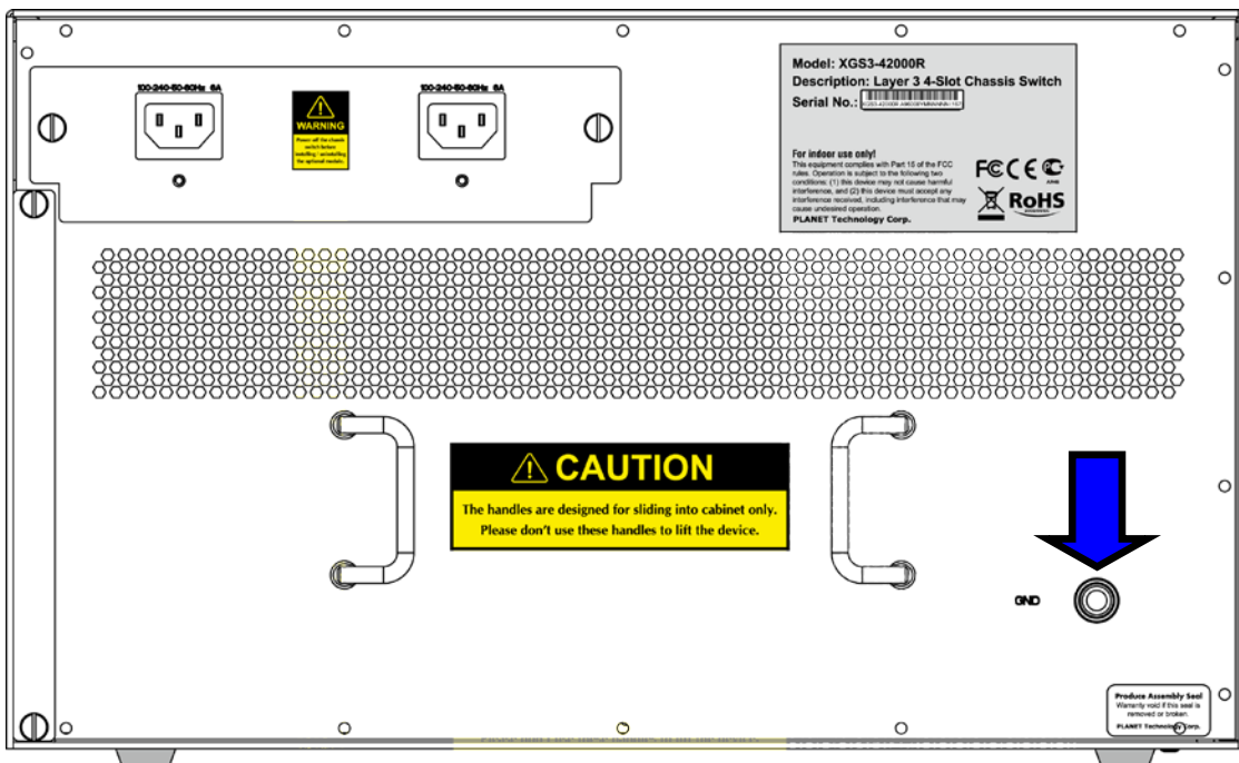
Figure 2-2-4 grounding posts
