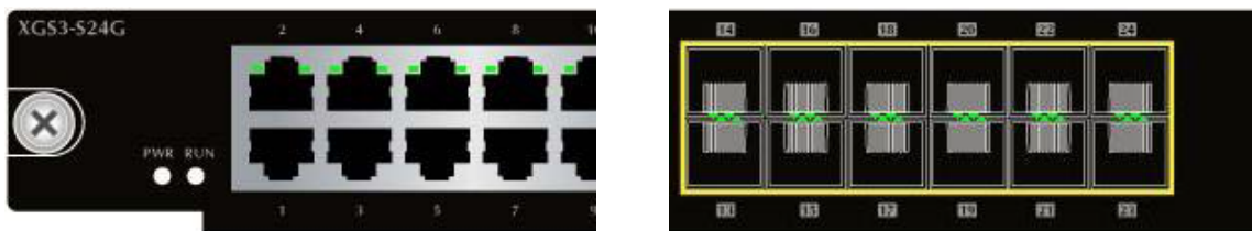
Figure 2-1-8 XGS3-S24G LED panel
