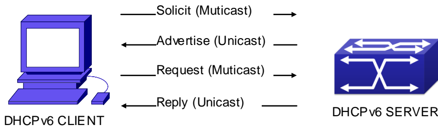
Figure 29-1-1 DHCPv6 negotiation
