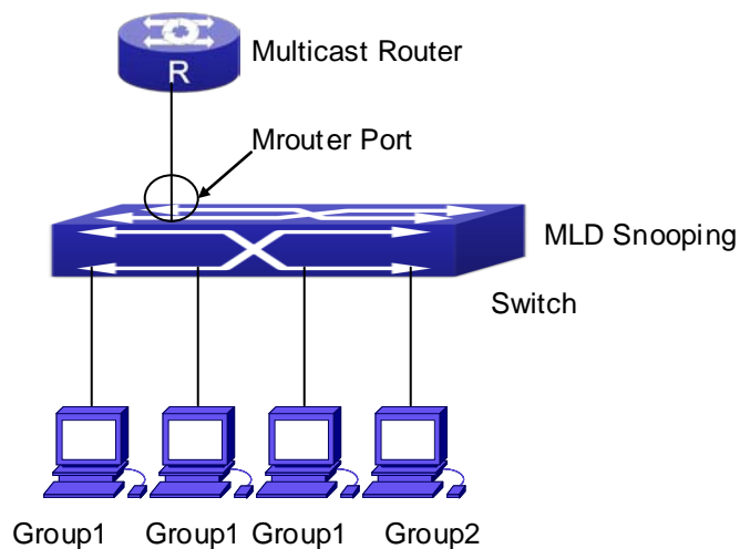
Figure 44-7-1 Open the switch MLD Snooping Function figure
