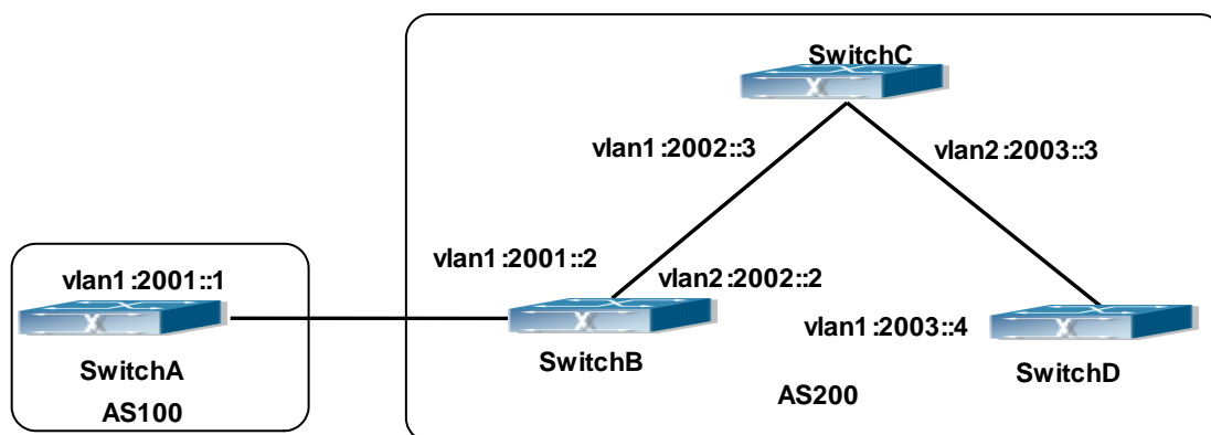
Figure 40-3-1 BGP Network Topological Map
