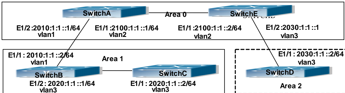
Figure 38-3-1 Network topology of OSPF autonomous system
