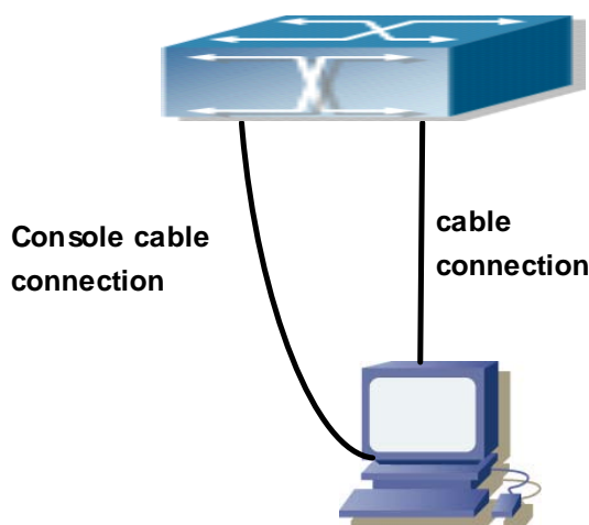
Figure 4-5-1 Typical topology for Chassis Switch upgrade in BootROM mode
