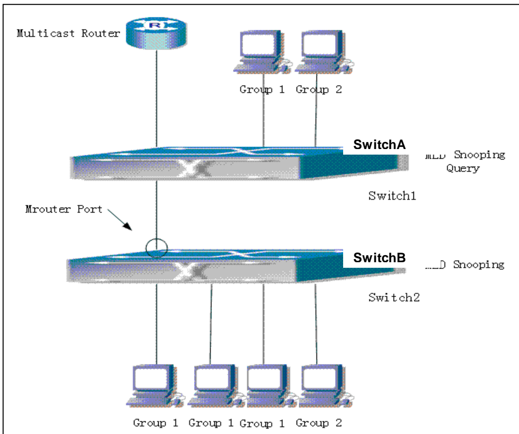
Figure 4-7-2 Switch as MLD Querier Function figure
