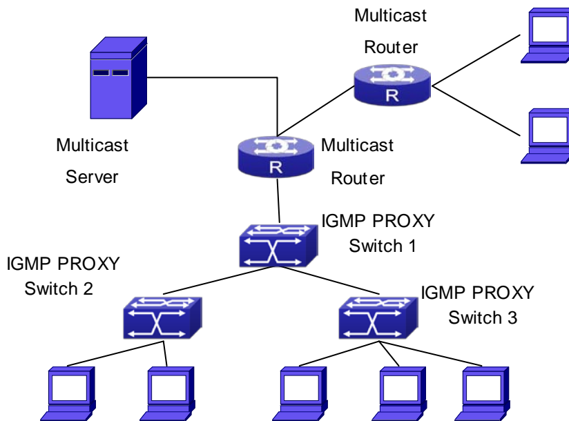
Figure 43-11-1 IGMP Proxy Topology Diagram
