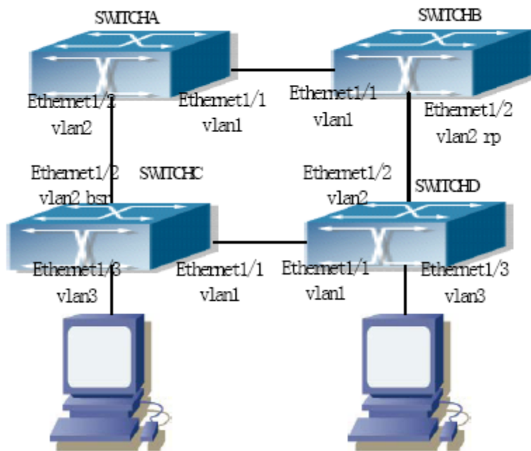
Figure 46-3-1 PIM-SSM typical environment
