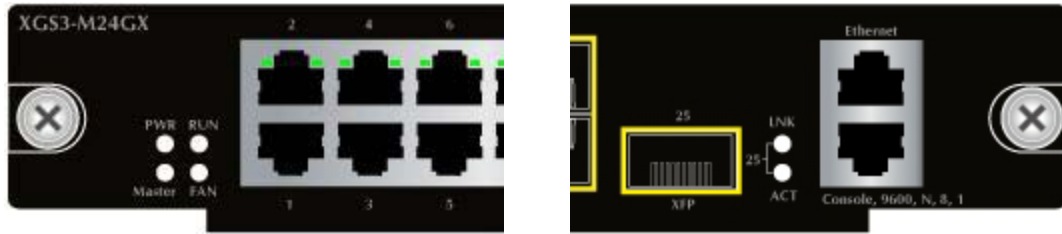
Figure 2-1-4 XGS3-M24GX LED panel
