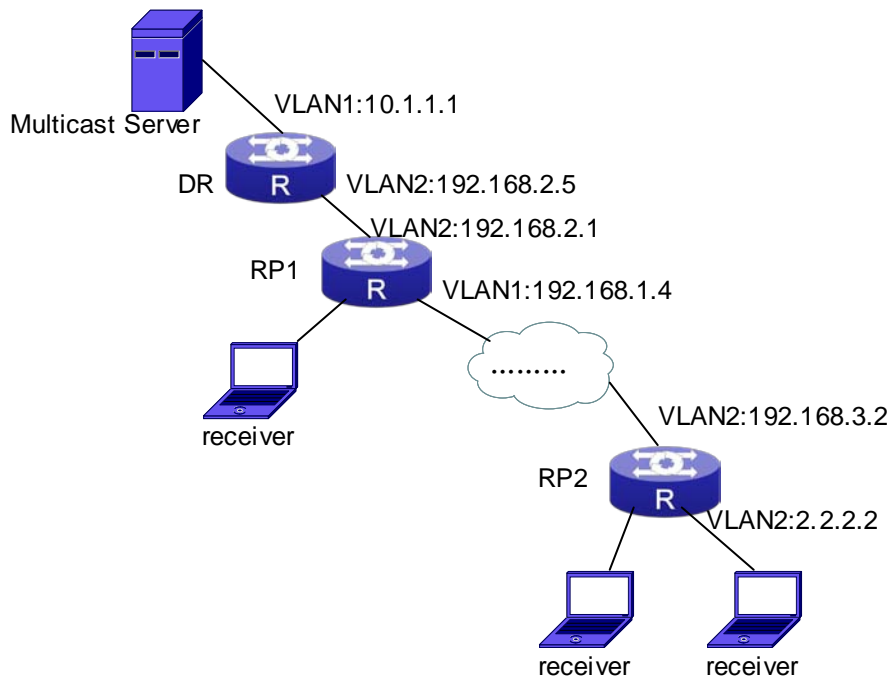
Figure 43-5-1 The ANYCAST RP v4 function of the router
