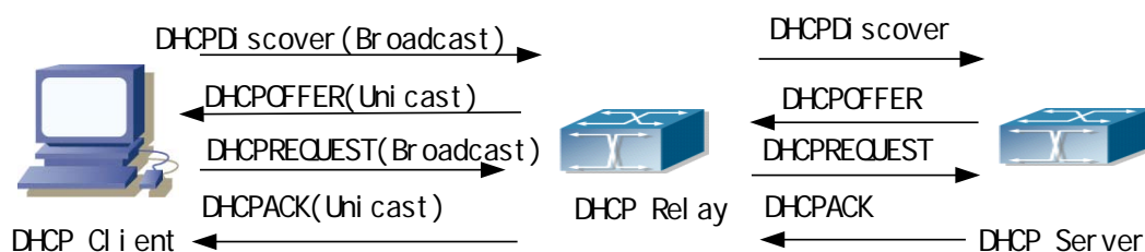
Figure 28-3-1 DHCP relay
