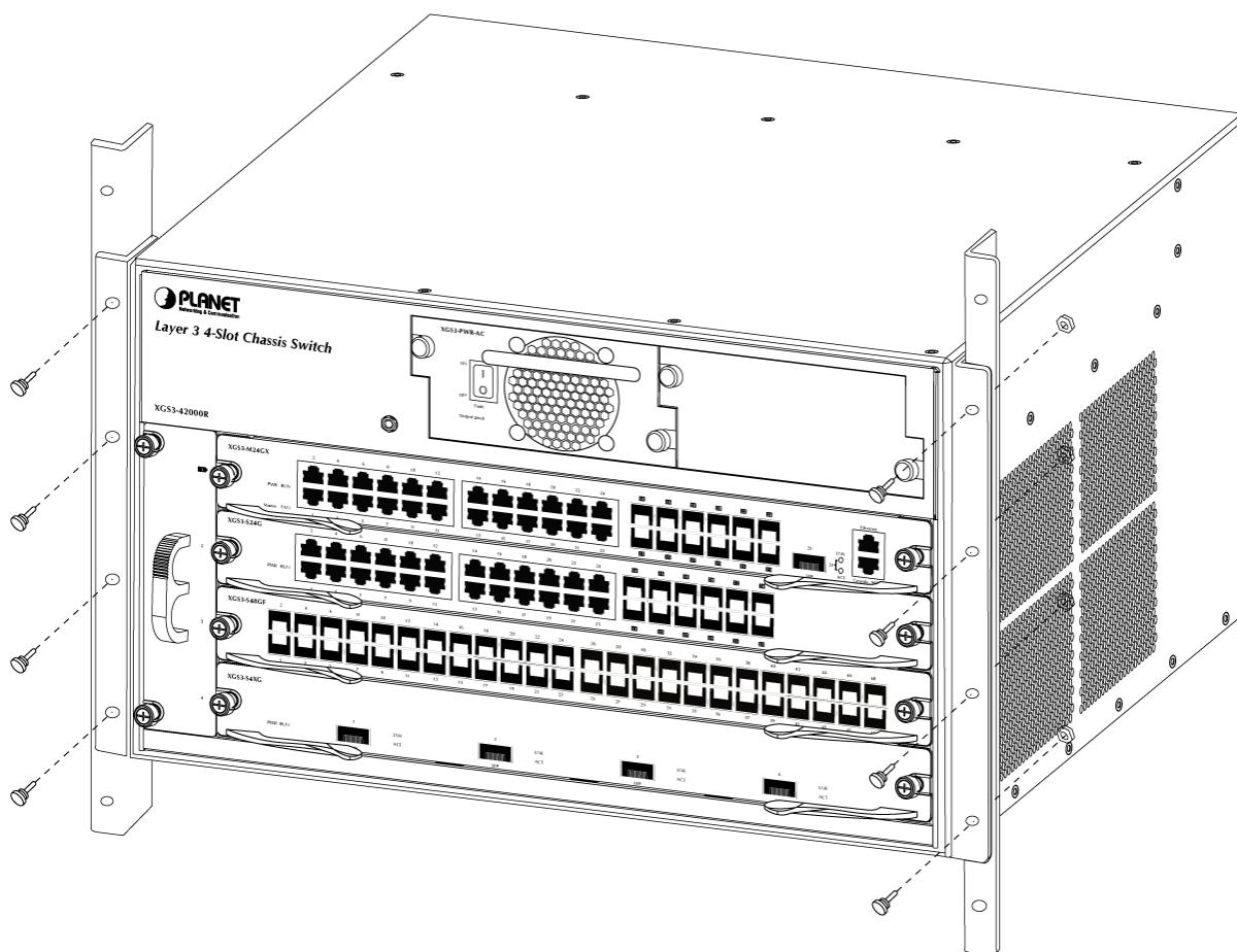
Figure 2-2-3 Mounting Chassis Switch in a Rack
