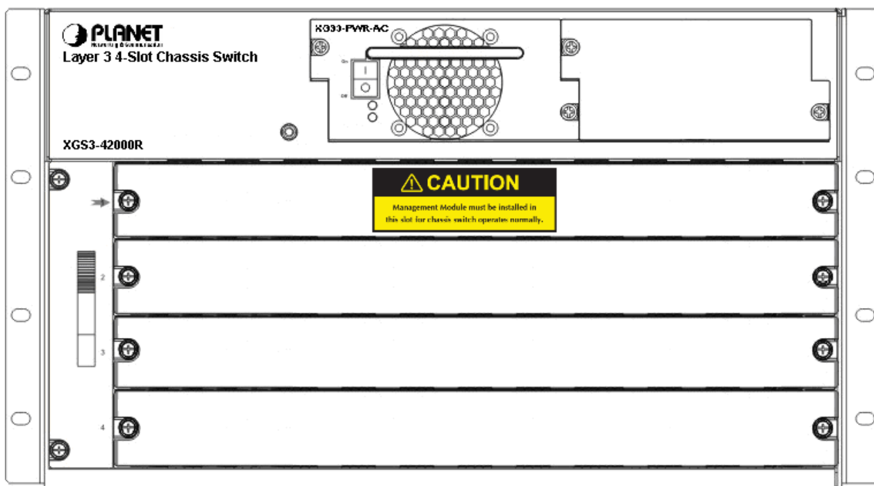
Figure 2-1-1 XGS3-42000R front panel
