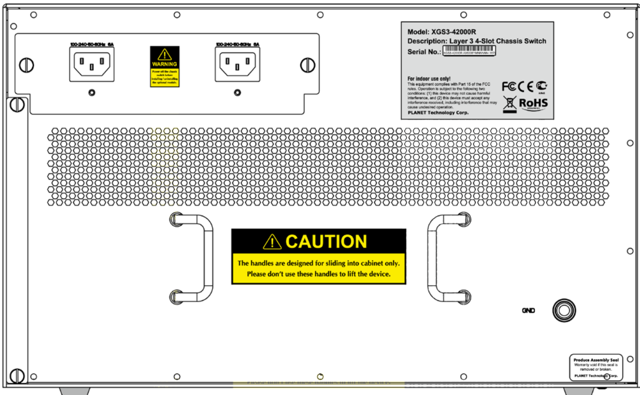
Figure 2-1-2 XGS3-42000R rear panel
