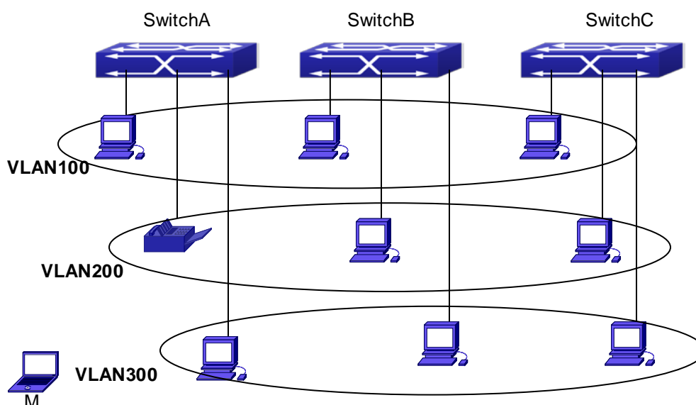
Figure 14-5-1 Typical topology application of dynamic VLAN
