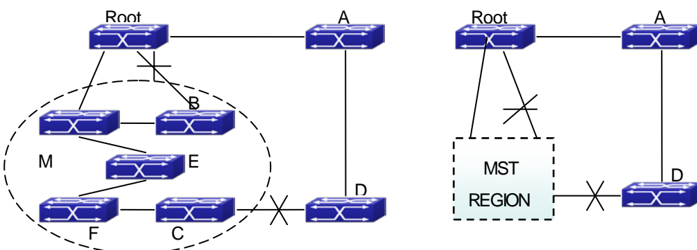
Figure 16-1-1 Example of CIST and MST Region
