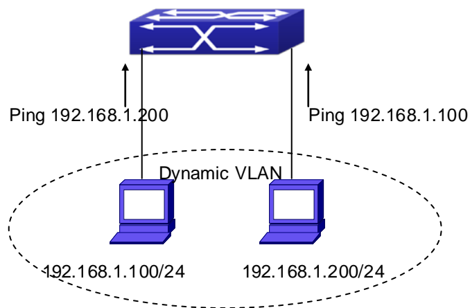
Figure 14-5-2 Dynamic VLAN Troubleshooting
