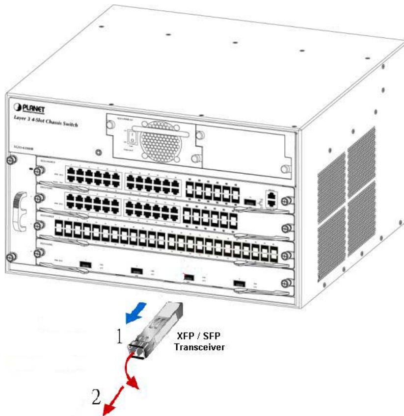
Figure 2-2-11 Pull out the SFP / XFP transceiver
