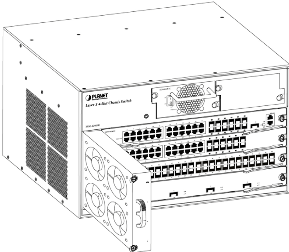
Figure 2-2-7 Installation and Removal the Fan Tray
