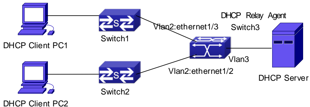
Figure 30-3-1 A DHCP option 82 typical application example
