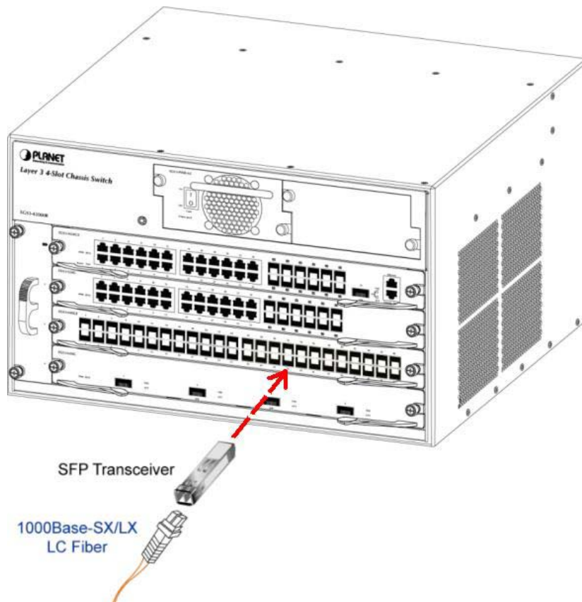
Figure 2-2-9 Plug-in the SFP transceiver
