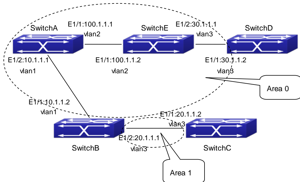
Figure 37-3-1 Network topology of OSPF autonomous system
