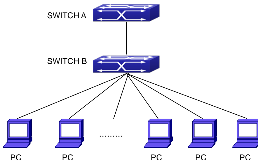
Figure 48-3-1 The Number Limitation of Port, MAC in VLAN and IP Typical Configuration Example
