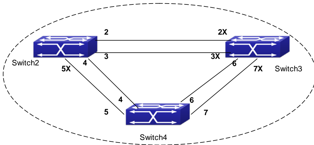
Figure 16-3-4 The Topology Of the Instance 4 after the MSTP Calculation
