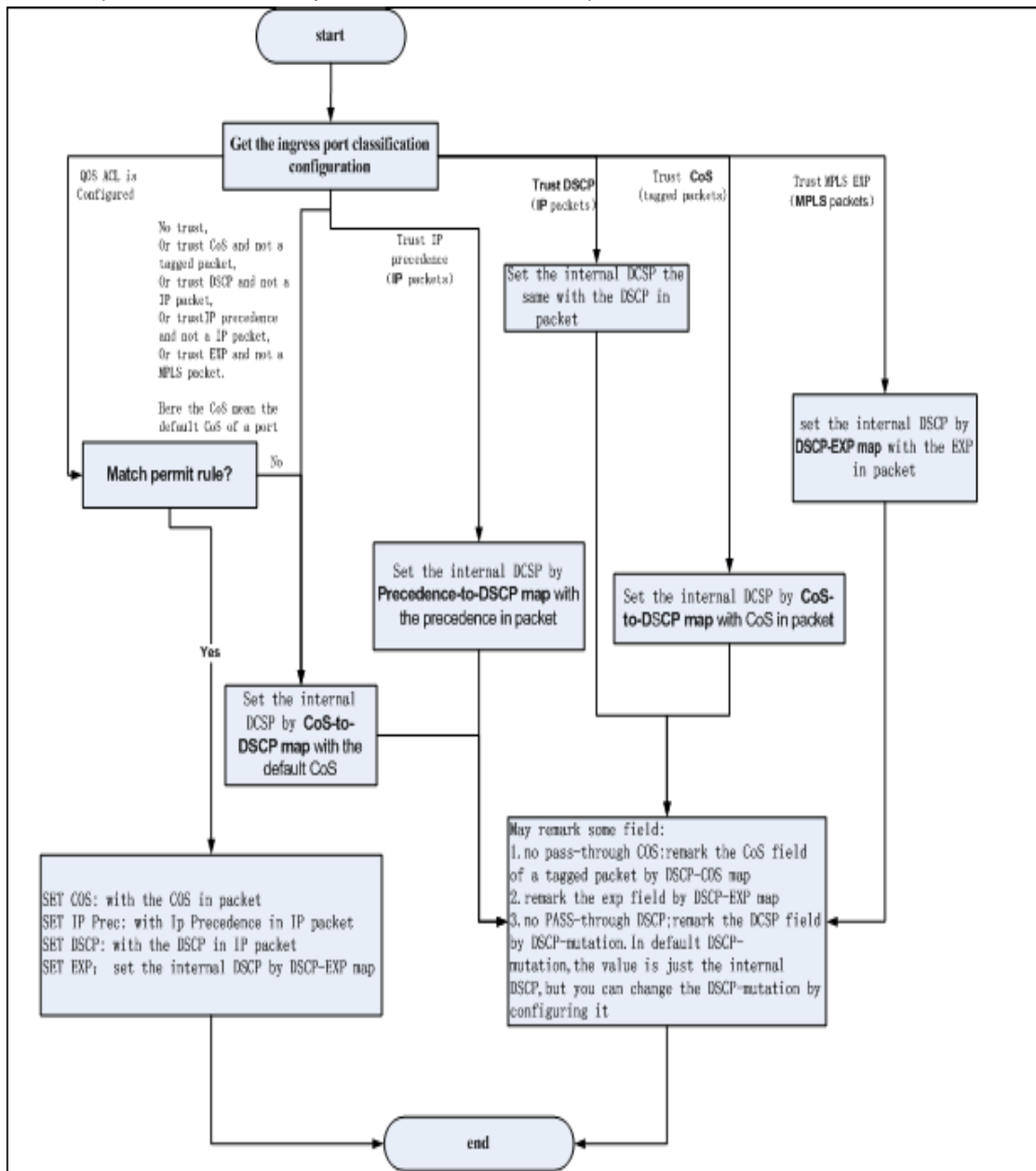
Figure 17-1-4 Classification process
