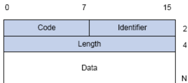
Figure 47-1-4 the Format of EAP Data Packets
